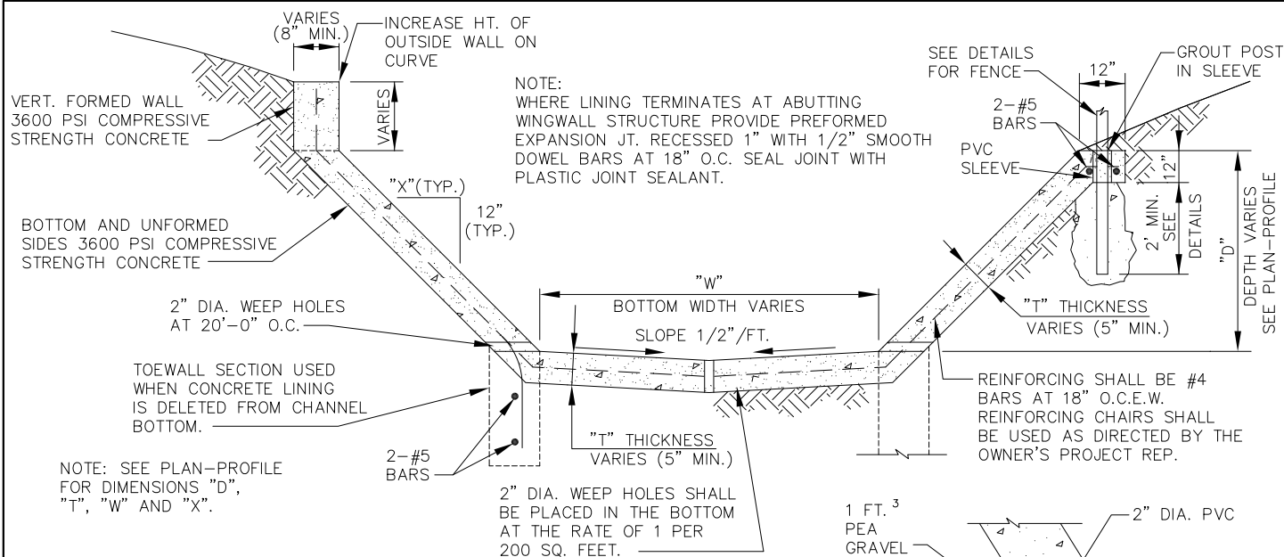
TYPICAL TRAPEZOIDAL SECTION
