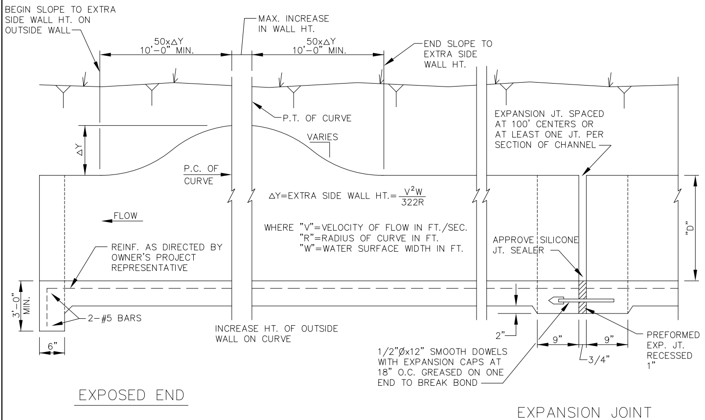
DETAILS OF REINFORCED CONCRETE CHANNEL LINER
