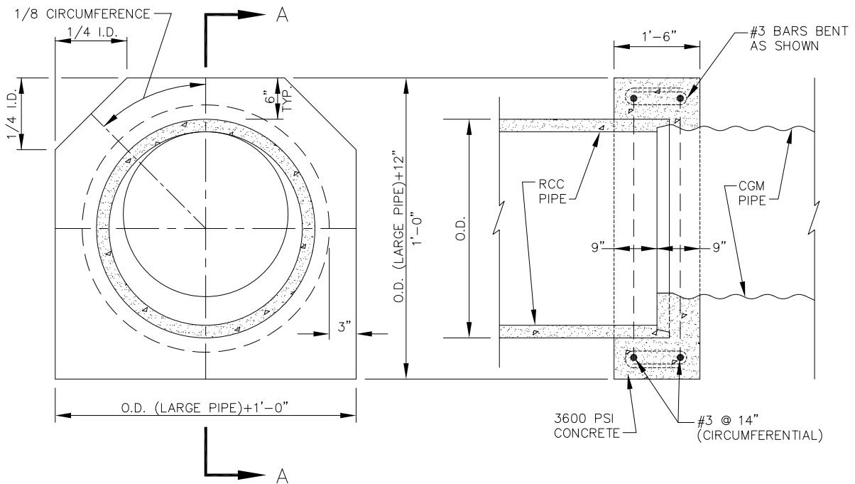
COUPLING OF RCCP TO CGMP
