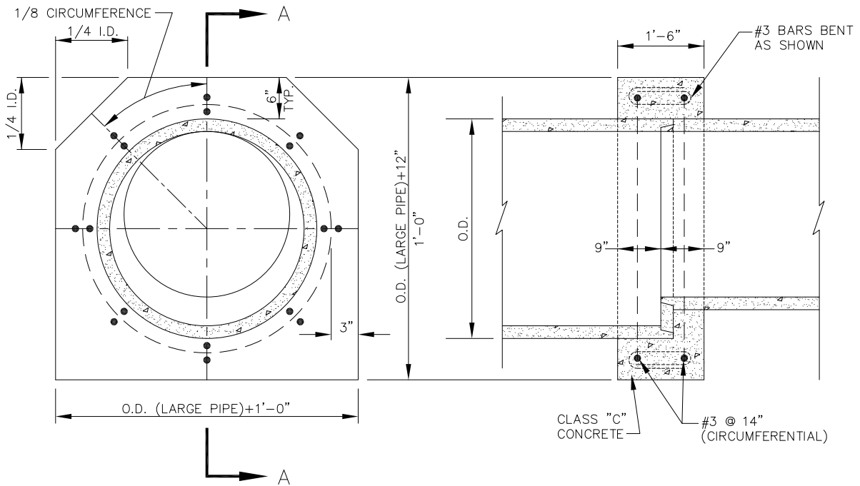
COUPLING OF R.C.C. PIPES OF DIFFERENT DIAMETERS
